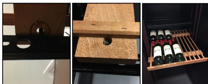
Clayette coulissante
